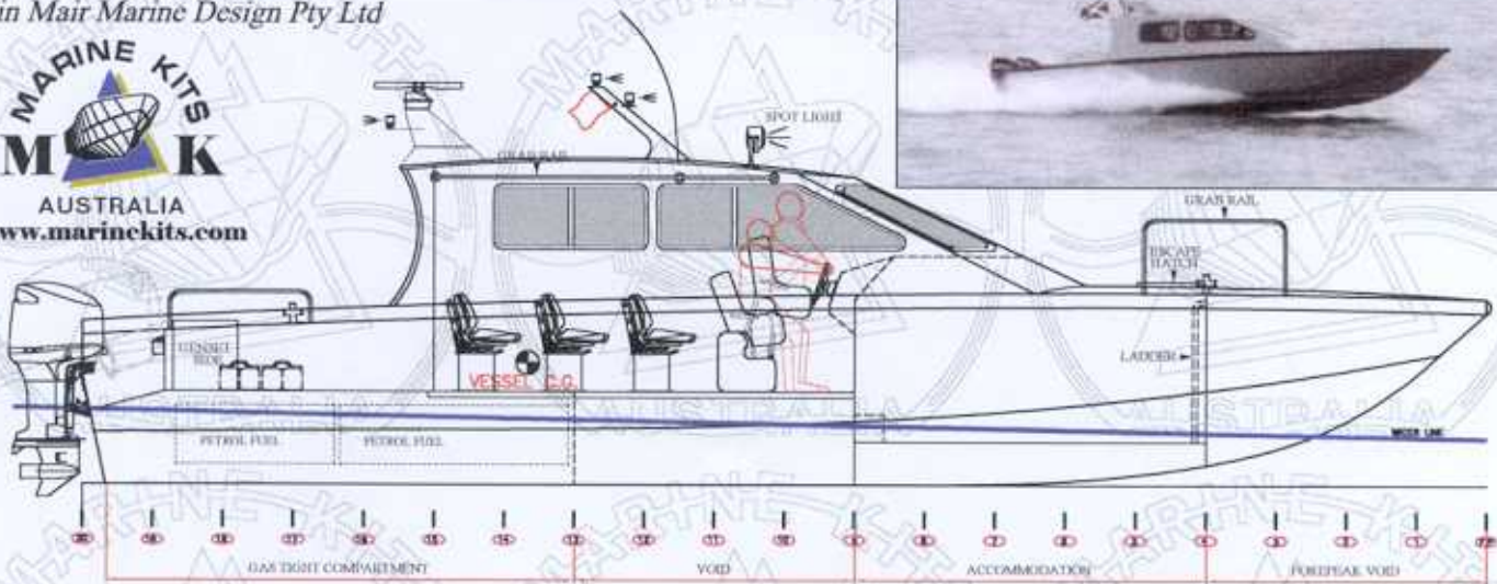
OUTBOARD PROFILE
